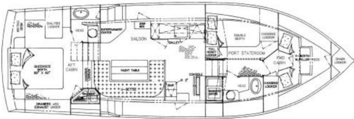
GB 42 M/YACHT ARRANGEMENT PLAN
